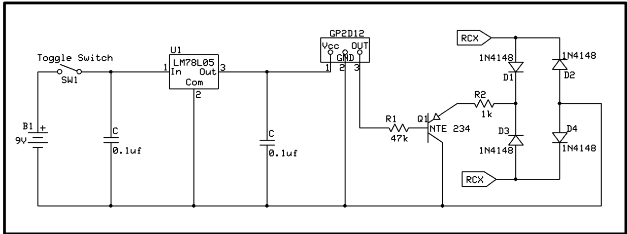
Figure 6. Distance sensor circuit.
